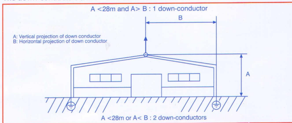
(Figure 1) - Number of down-conductors
